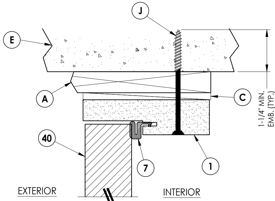
3 6 VERTICAL CROSS SECTION Shown w/ 1X sub-buck Outswing
