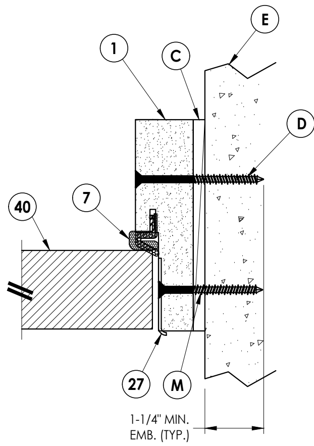
2 7 HORIZONTAL CROSS SECTION Shown Direct to Masonry Outswing
