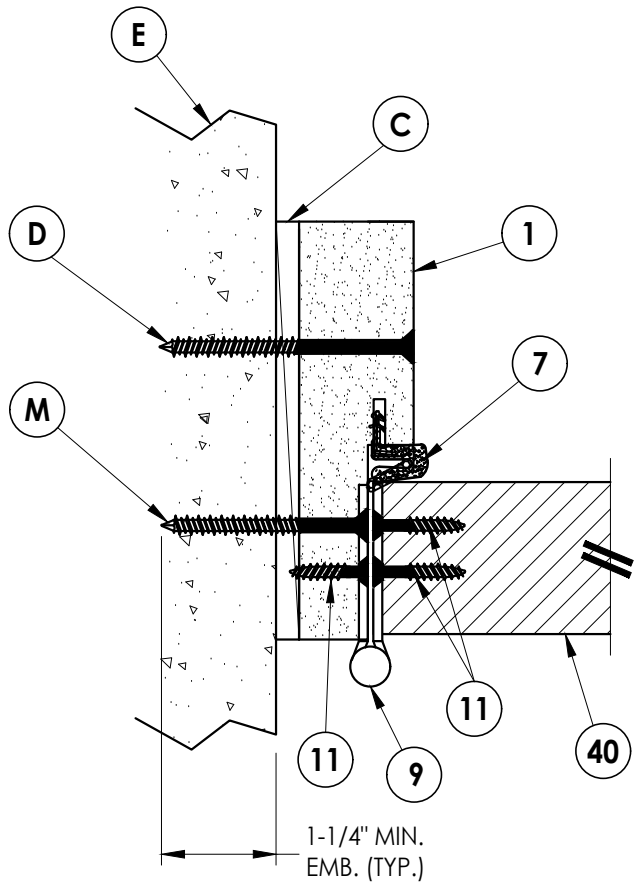
1 7 HORIZONTAL CROSS SECTION Shown Direct to Masonry Outswing
