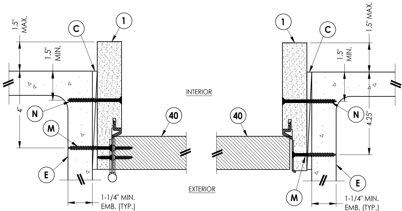
4 8 HORIZONTAL CROSS SECTION Shown Direct to Masonry Outswing only w/ 6-9/16" jamb
