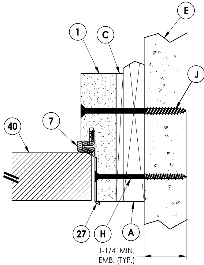
2 6 HORIZONTAL CROSS SECTION Shown w/ 1X sub-buck Outswing
