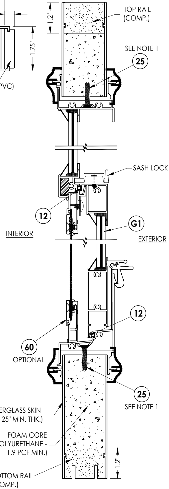
2 2 VERTICAL CROSS SECTION
